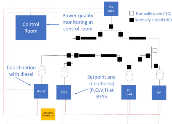
Figure 3. The structure of the system in the IEEE Std 2030.7-2017 [3]
