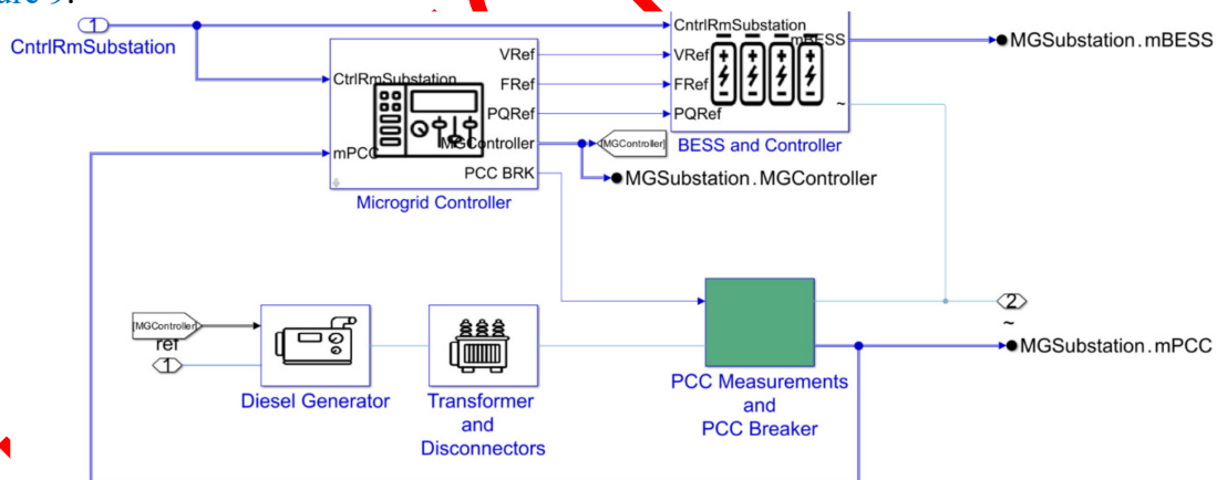
Figure 9. The model of Diesel Substation – BESS - Microgrid Controller in MATLAB/Simulink®(R2023b)
