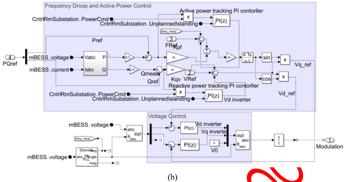
Figure 8. The BESS and its controller in MATLAB/Simulink® (R2023b) (a); and the BESS module and its BESS converter in MATLAB/Simulink®(R2023b) (b)
